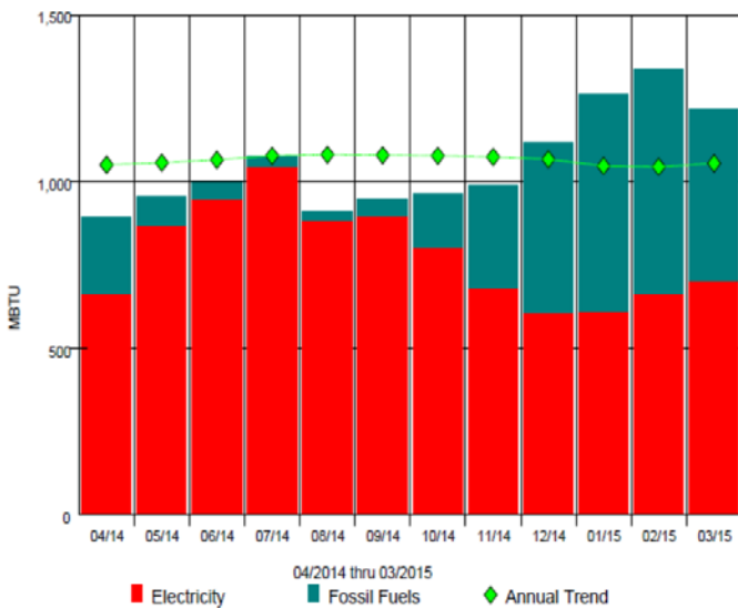
Energy Use Graph - Monthly and Annual Trend for Monticello High
