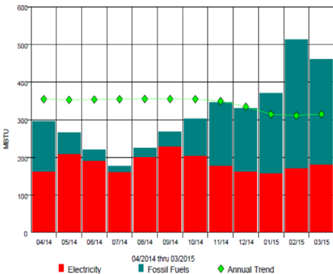
Energy Use Graph - Monthly and Annual Trend for Cale Elementary
