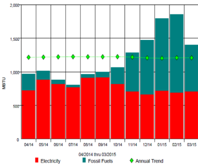
Energy Use Graph - Monthly and Annual Trend for Albemarle High
